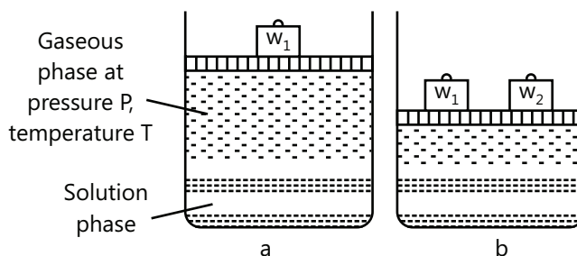
Figure 20.2: Demonstrating the effect pressure on solubility of a gas in liquid
