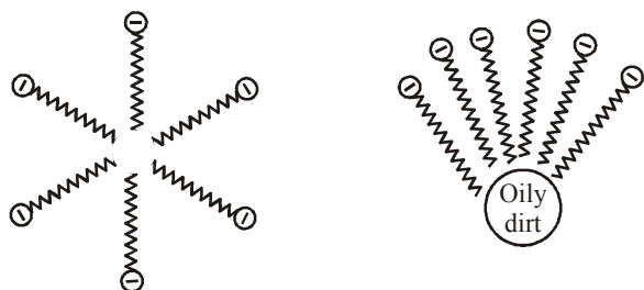
Micelle formed by detergent molecules in water. The hydrocarbon tail sticks to oily dirt
