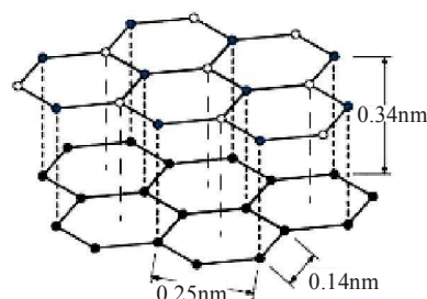
The structure of graphite
