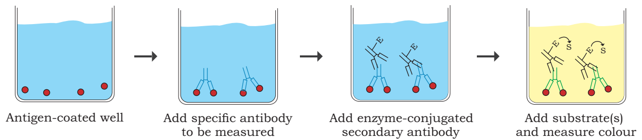
Fig. 12.6: Indirect ELISA
