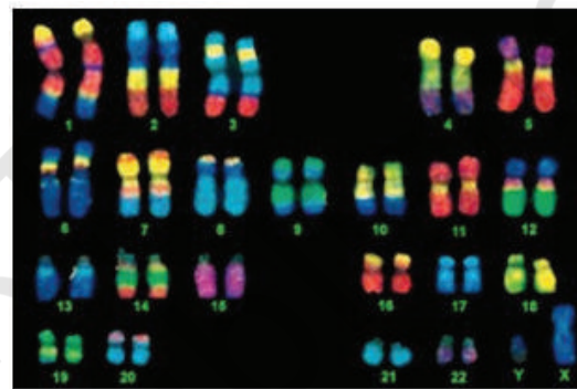
Fig. 12.16: Chromosome painting
