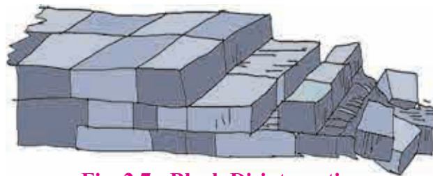
Fig. 2.7 : Block Disintegration
