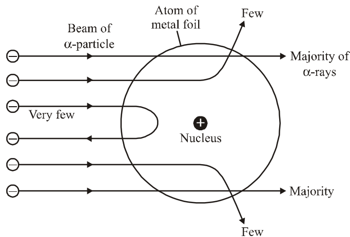
Fig. Scattering of \alpha -particles
