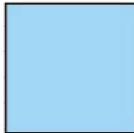
A square
