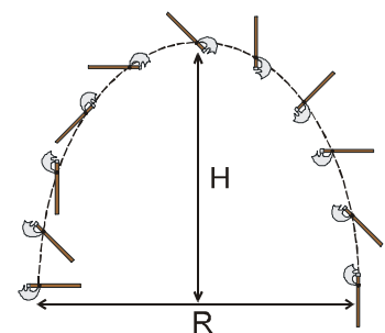
The motion of axe is complicated but the COM is moving in a parabolic motion.
