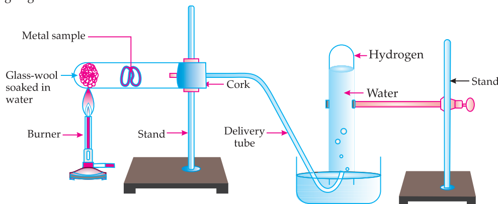
Reaction of metal with steam
