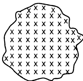
Absorption
