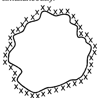
Adsorption
