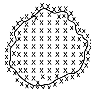
Sorption
