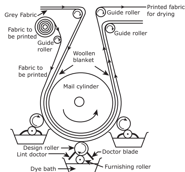
Figure 3.15 Schematic Diagram for Roller Printing
