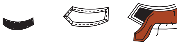
Figure 9.12 Steps in Construction of Contour Belt
